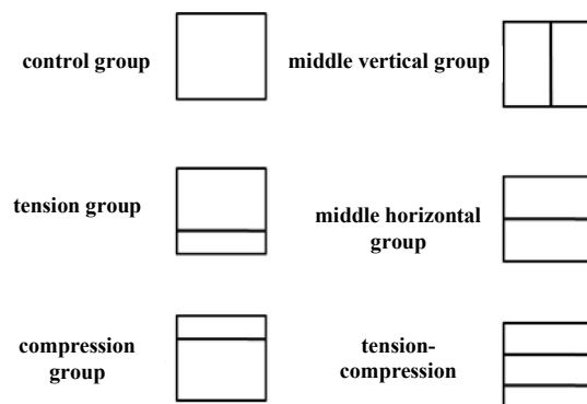
Fig.2: Schematic aspect of cross-section of specimen
