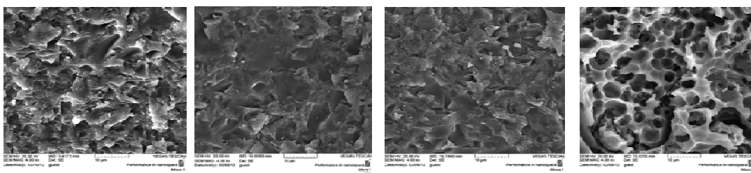
Figure 2. SEM analysis of the mode of failure of samples in groups 1 to 4 from right to left (1000X magnification)
