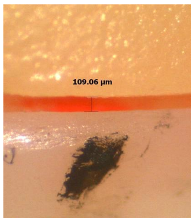
Figure 4. Gap measurement using stereomicroscope at \times 35 magnification.
